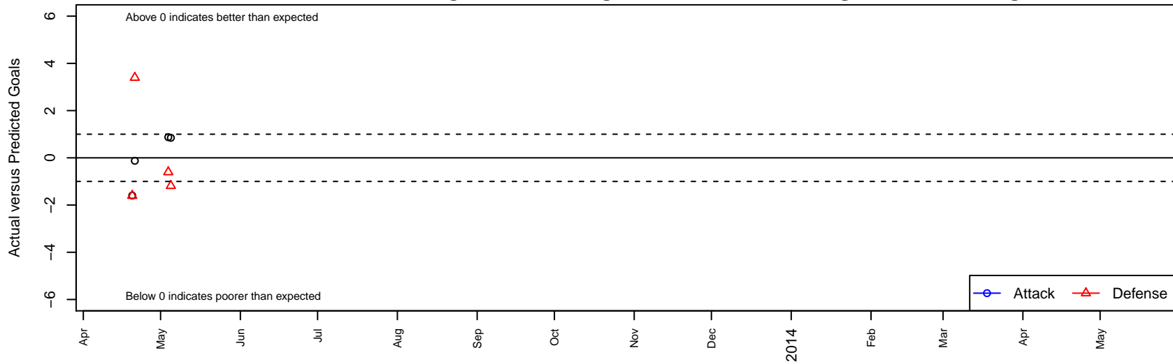
OSA Alliance B98 Dots are actual minus expected GF (blue circles) and GA (red triangles). Blue line is smoothed change in attack strength. Red is smoothed change in defense strength.
